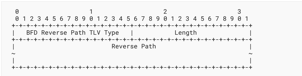
Figure 1: BFD Reverse Path TLV
